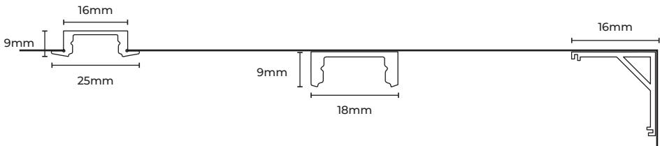
Recessed
